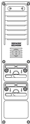
WFD Weatherproof Digital U p0 Call Stations, 2 Double Toggle Art.-No. 1 639 9 With 25W additional amplifier Art.-No. 1 636 6
